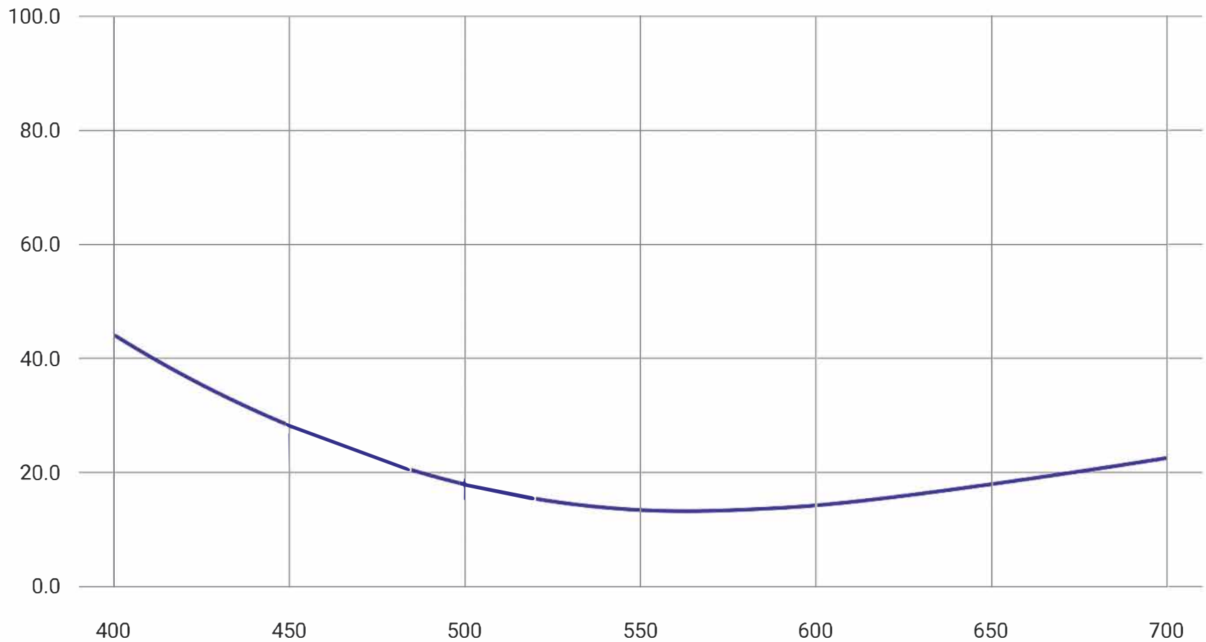
Reflectance (%) vs. Wavelength (nm)
