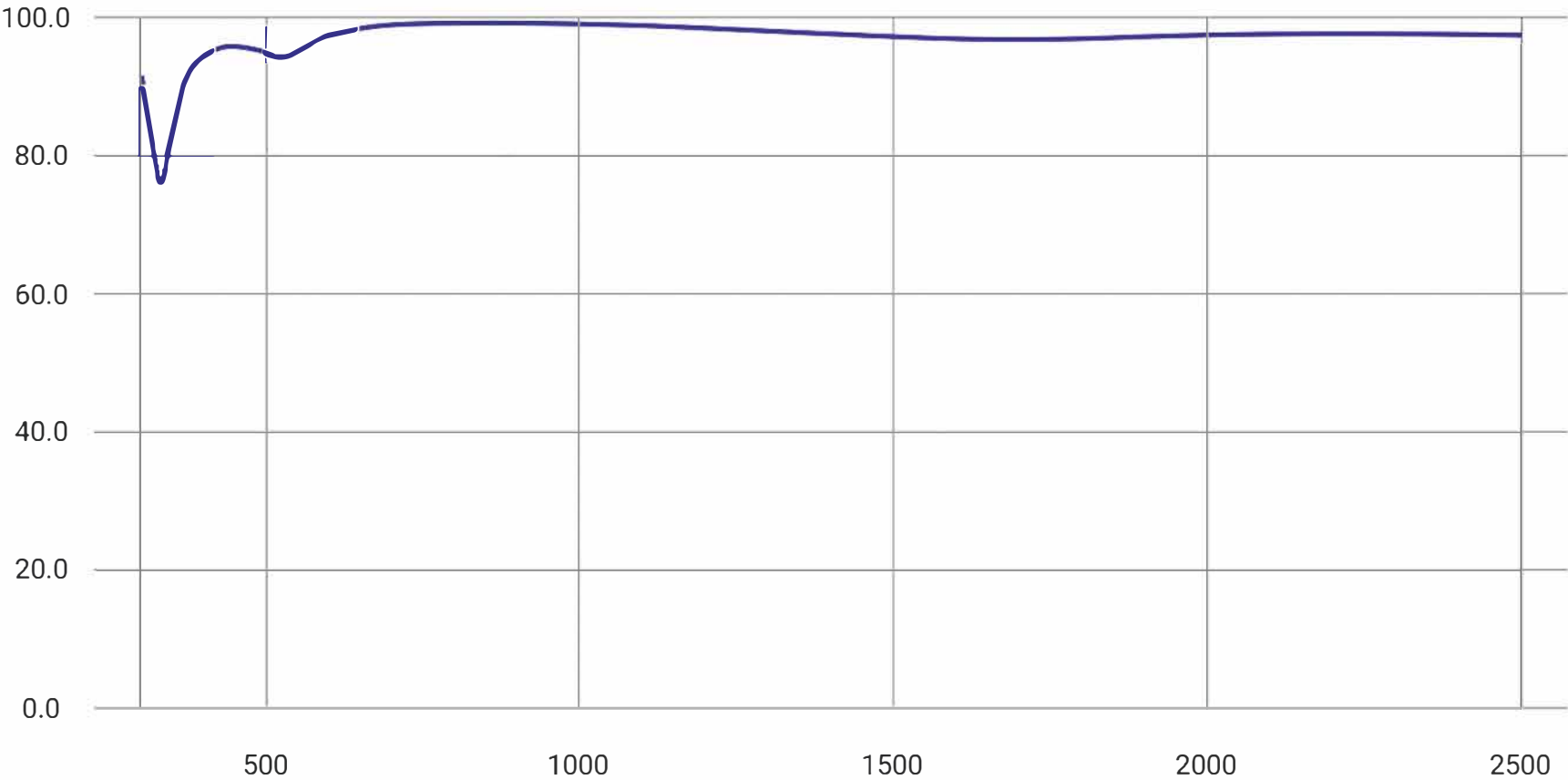
Reflectance (%) vs. Wavelength (nm)
