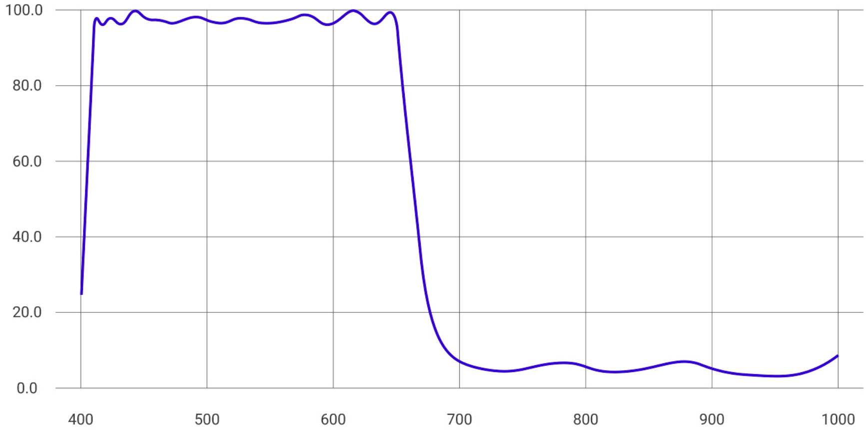
Transmittance (%) vs. Wavelength (nm)
