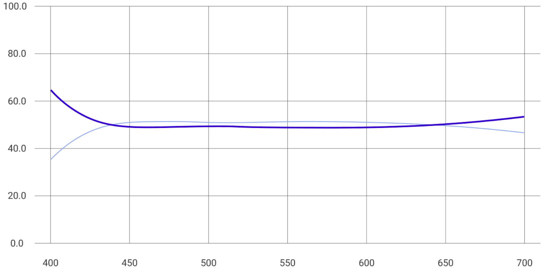
Transmittance (%) and Reflectance (%) vs. Wavelength (nm)
